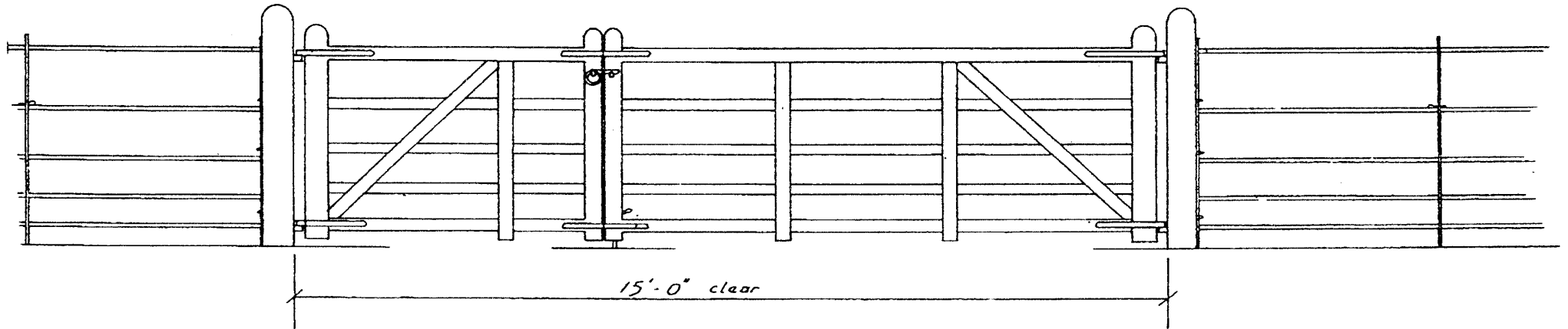
The Cotswold Gate & Wicket with Estate Railing
