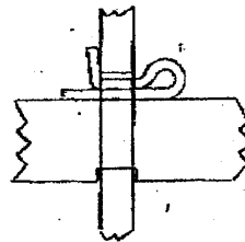
Top 25x6 RSF Rail c/w Notch Detail (All Posts)
