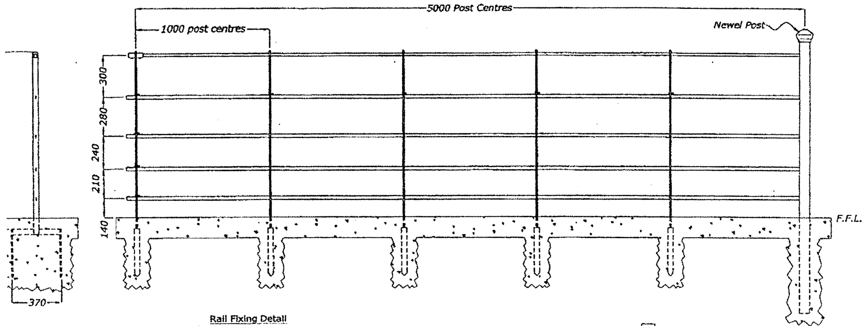
Rail Fixing Detail
