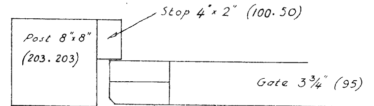
Plan of Stop
