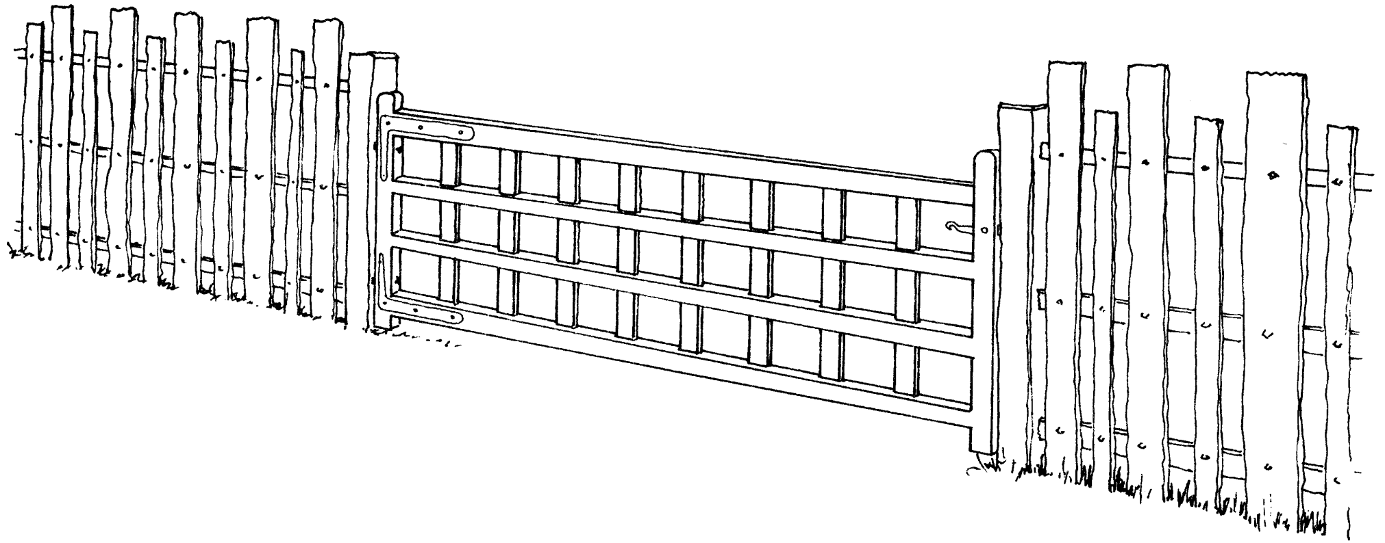
Norman Park Paling of Cleft Oak & Tudor Field Gate
